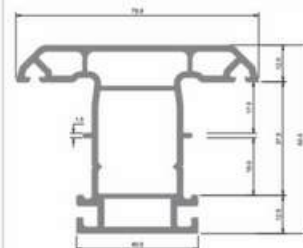
Prominace UPVC Casement Mullion YTB 77 105
