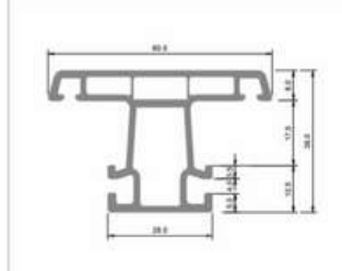
Simta UPVC Sliding & Casement Mullion YTB 77 106
