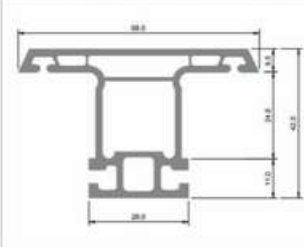
Prominace UPVC Sliding & Casement Mullion YTB 77 108
