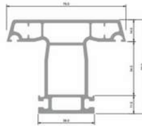
Prominace UPVC Casement Mullion YTB 77 105
