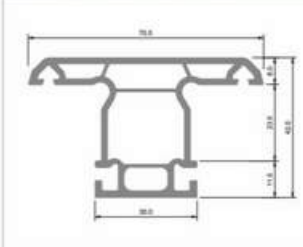
JPI UPVC Sliding & Casement Mullion YTB 77 109
