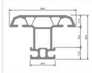
Prominace UPVC Sliding & Casement Mullion YTB 77 110
