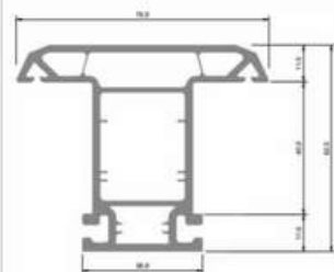
Prominace UPVC Casement Mullion YTB 77 104
