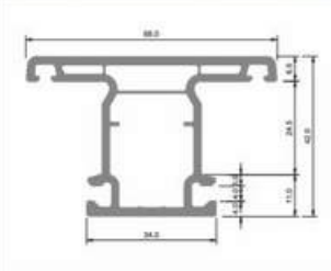
Kaka UPVC Sliding & Casement Mullion YTB 77 107
