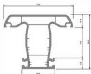
PSP UPVC Casement Mullion YTB 77 103
